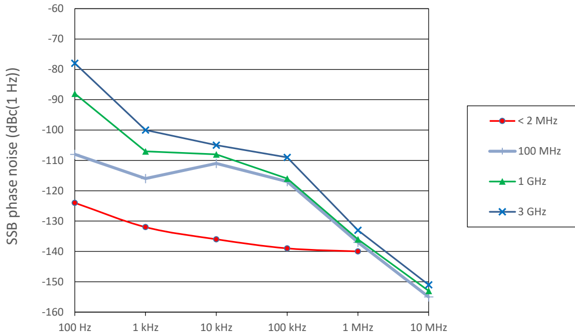
Typical phase noise at different center frequencies.
